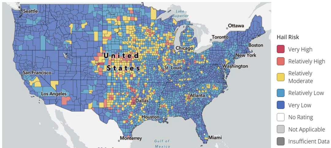
Figure 61: Hail Risk across the United States
