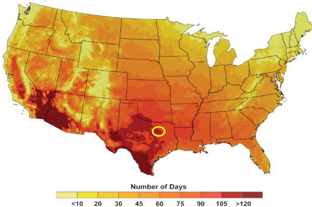
Figure 48: Average Number of Days Annually Expected to Exceed 100°F by the End of the Century 75
