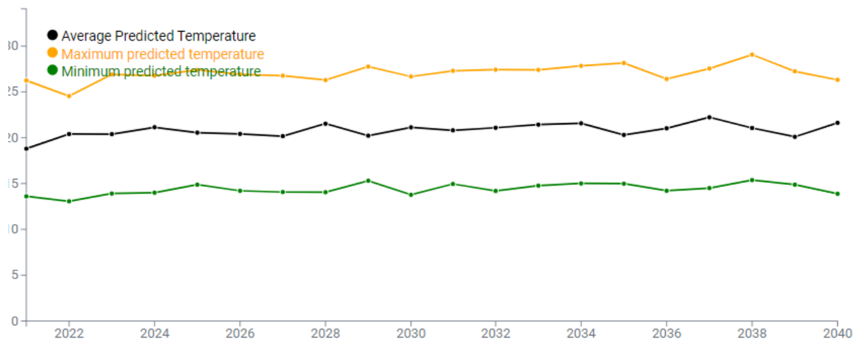
Figure 25: Climate Change Forecast, Future Climate Trends for Tarrant County, Texas 37
