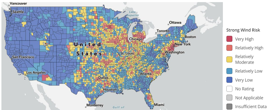
Figure 62: Strong Wind Risk across the United States
