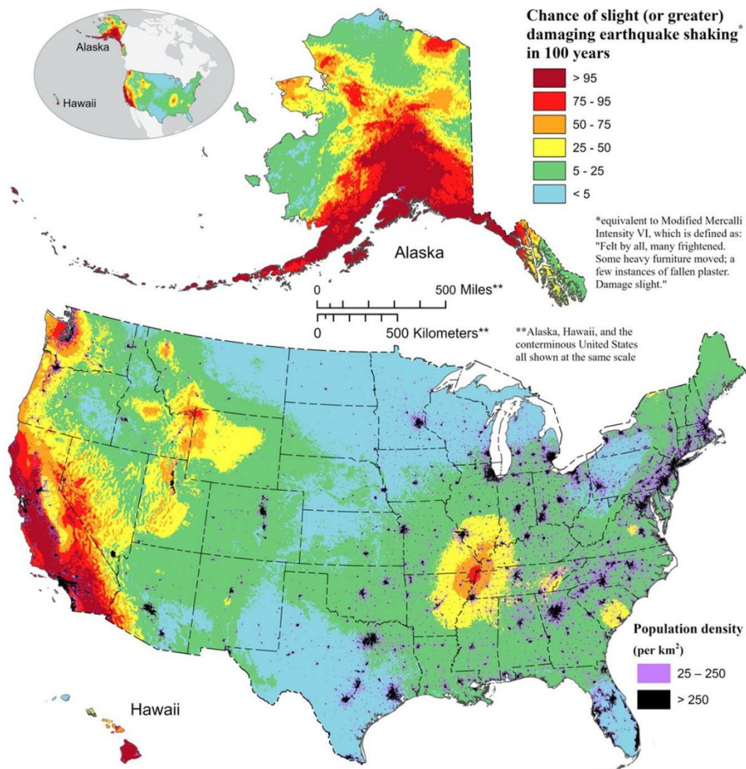
Figure 33: National Seismic Hazard Model
