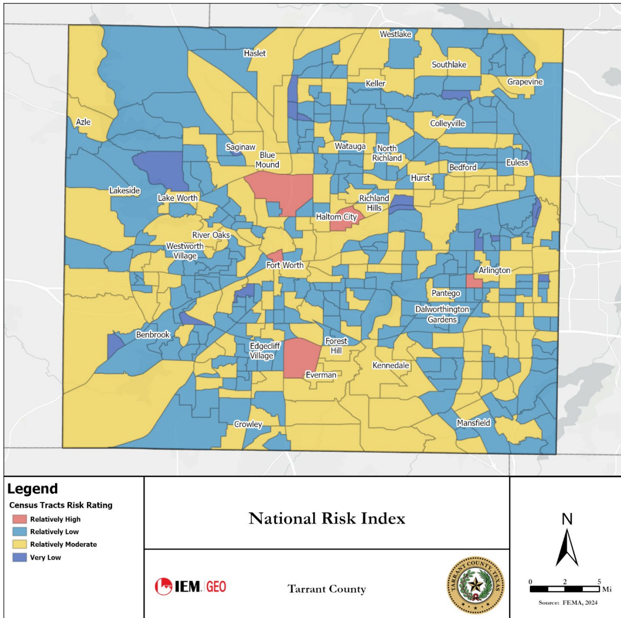
Figure 3: National Risk Index Score by Census Tract for Tarrant County
