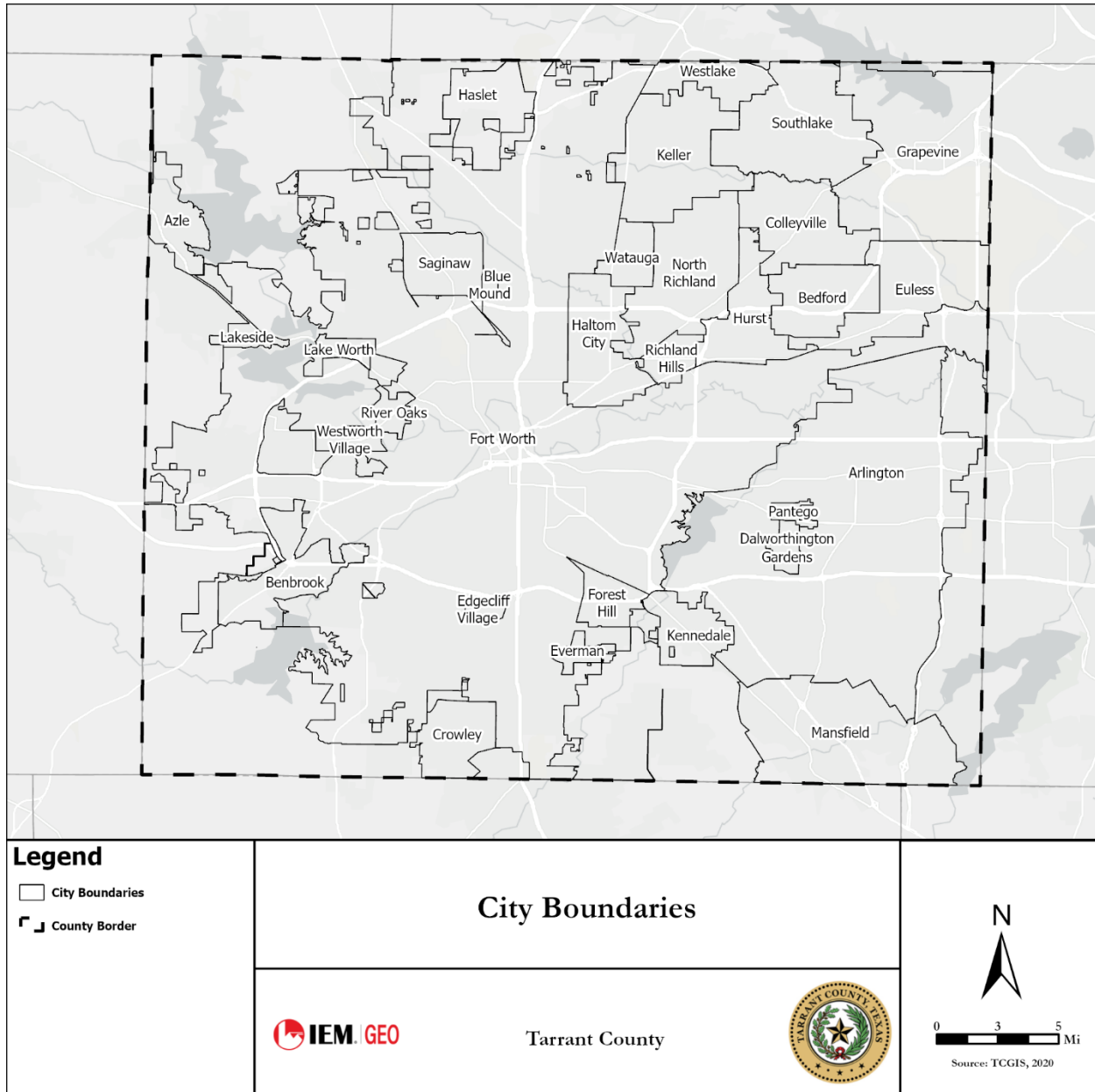
Figure 2: HazMAP Jurisdictions in Tarrant County
