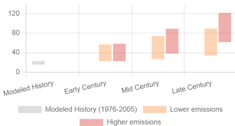
Figure 24: Effects of Higher and Lower Emissions on 100-Degree Days through 2100 33
