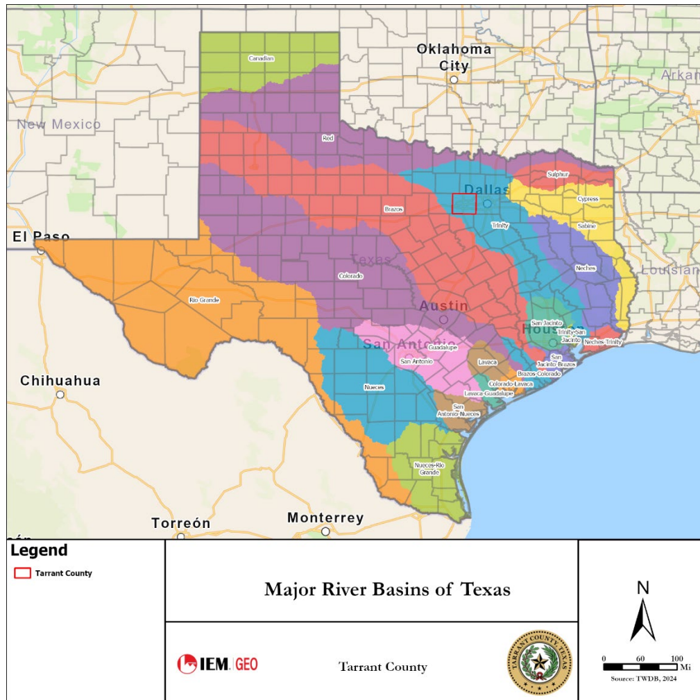
Figure 54: Major River Basins of Texas
